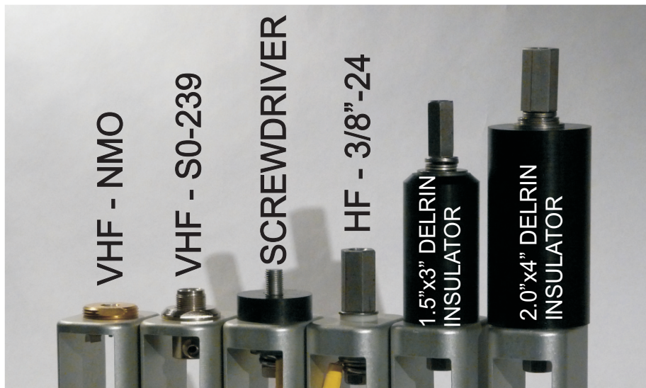
1.5" or 2.0" Delrin Screwdriver Antenna Adaptor
